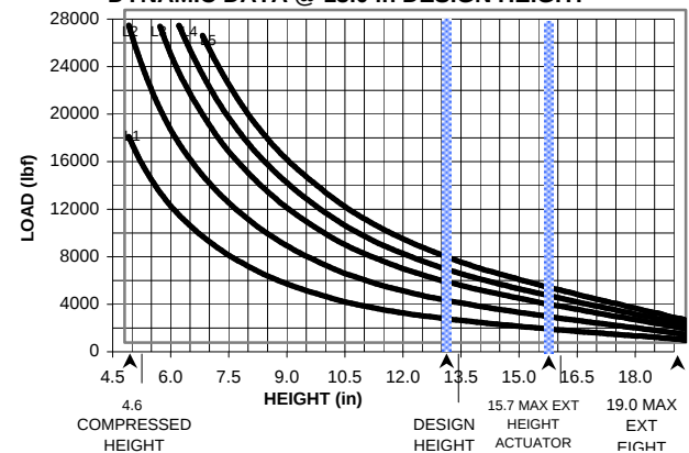
DYNAMIC DATA @ 13.0 in DESIGN HEIGHT
